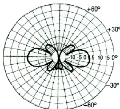
Diagrama de Radiación Vertical Vertical Radiation Pattern
